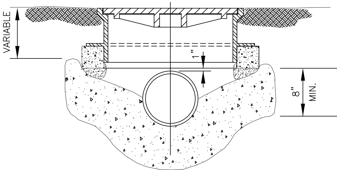
SHALLOW MANHOLE
